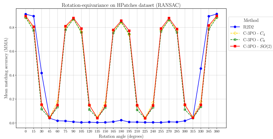
Fig. 3: Evaluation Rotation-Equivariance. We compare vanilla R2D2 model with our model variants that endow R2D2 with rotation-equivariance capabilities. At and around special rotations, SO(2) outperforms other variants but only marginally.
